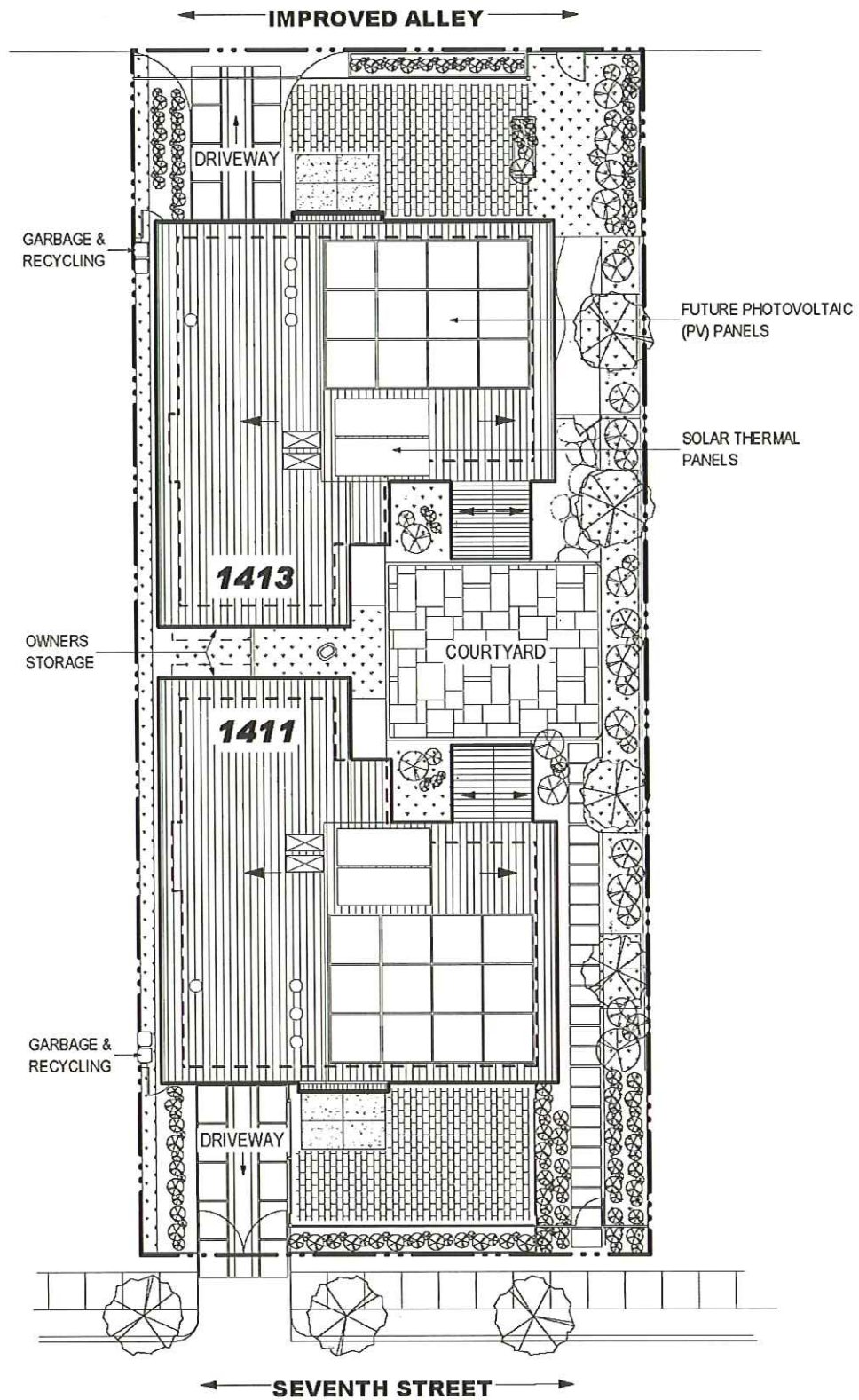
SITE PLAN
